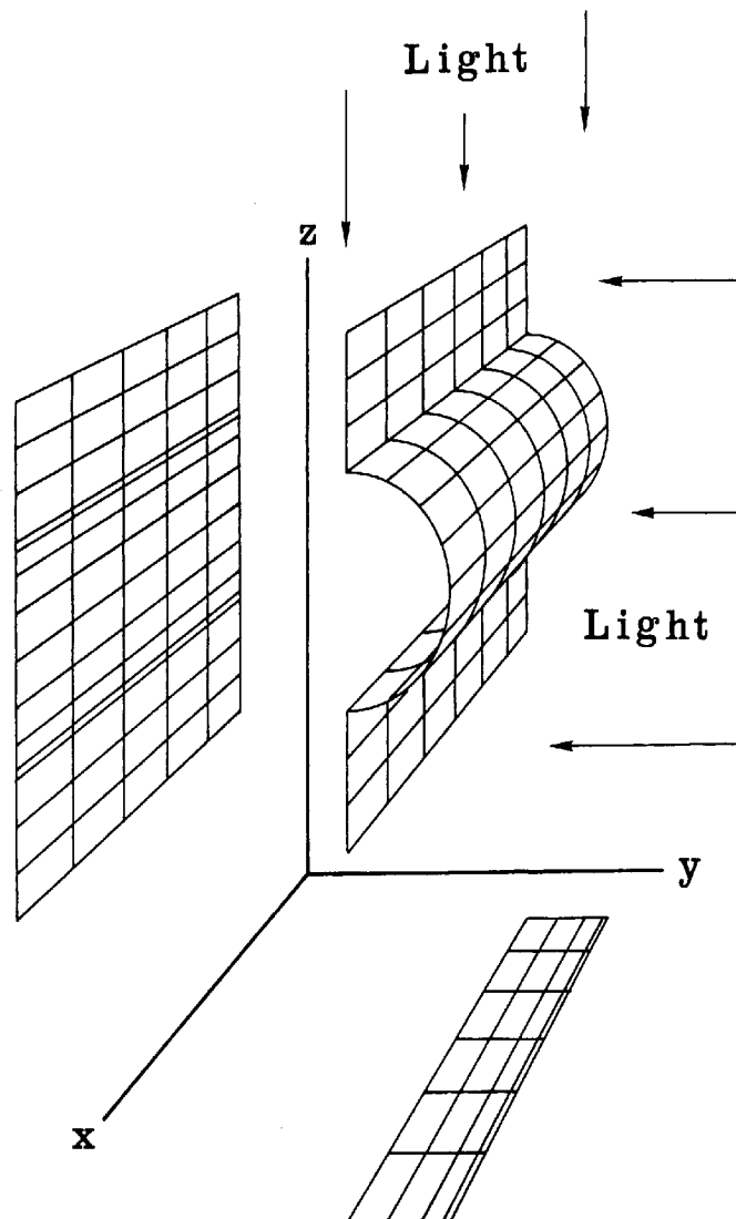
Fig.1. Metronic condensations in 3 dimensions
